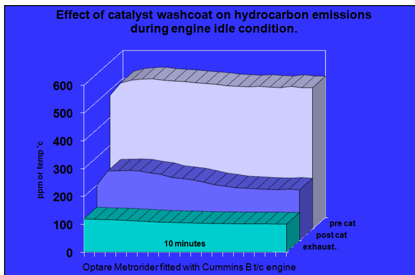
Hydrocarbon Reduction Performance AZ Diesel Oxidation Catalyst
