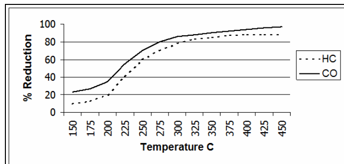
HC and CO Reduction Performance DZ Diesel Oxidation Catalyst
